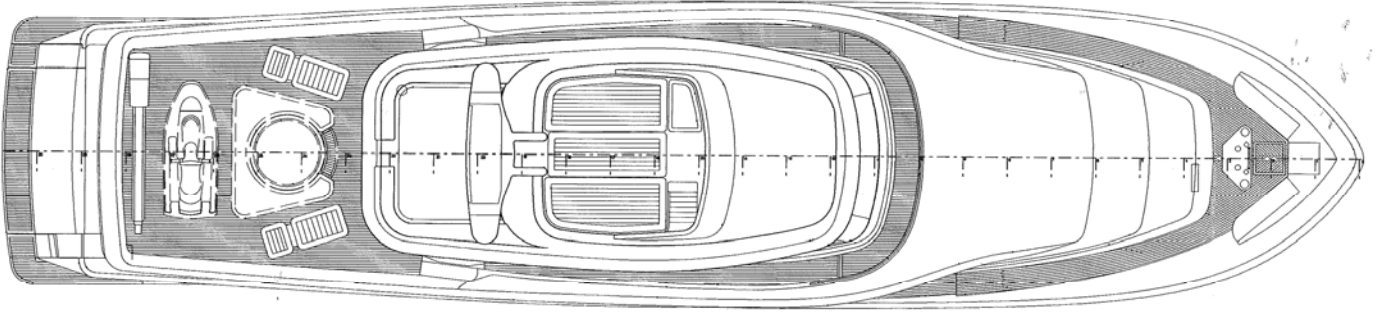
Upper Deck
